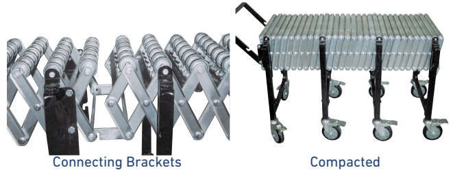
Connecting Brackets
